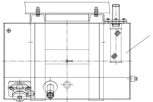
Fig. 9-6-1 SCS866LS OIL TANK SET
