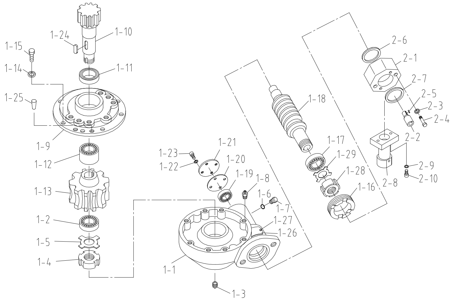
Fig. 2-3 SCS866LS SWING R/G SET
